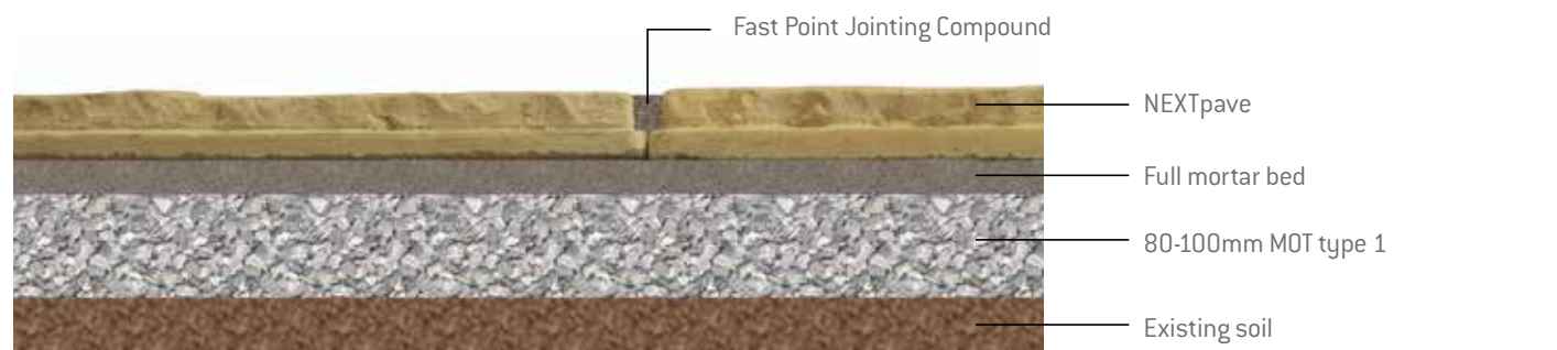
4. Install the engineered NEXTpave using the laying pattern
